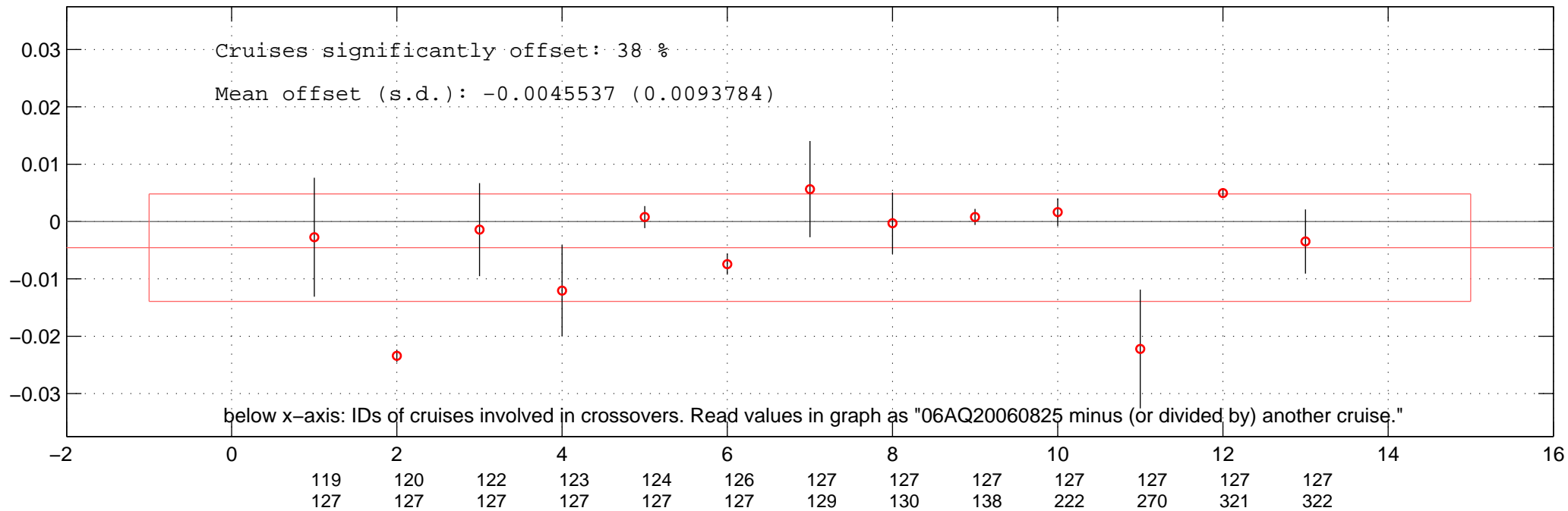
all additive offsets of SAL of 06AQ20060825 in Favourite-space.
