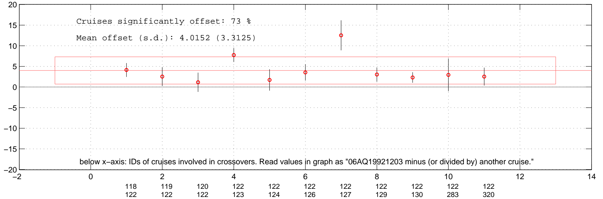
all multiplicative offsets of SIL of 06AQ19921203 in Favourite-space.
