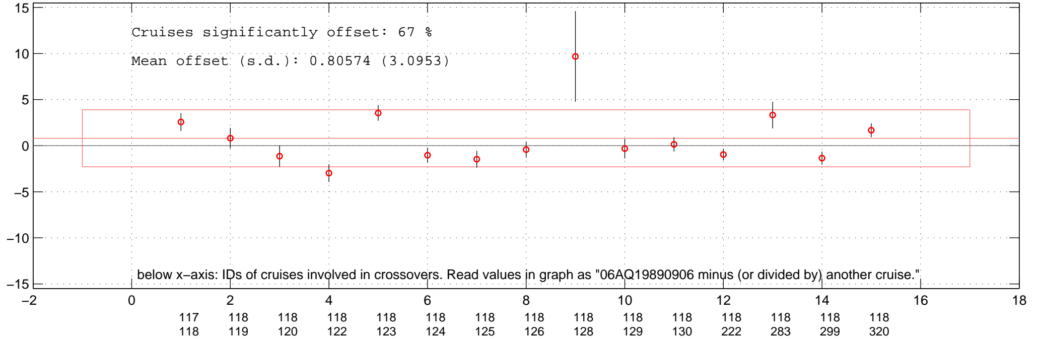
all multiplicative offsets of NO3 of 06AQ19890906 in Favourite-space.
