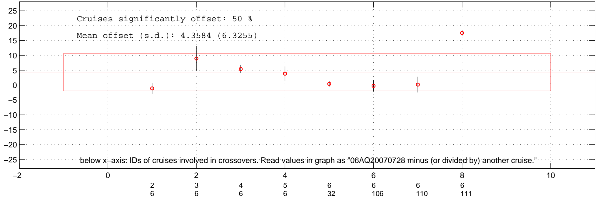
all multiplicative offsets of NO3 of 06AQ20070728 in Favourite-space.
