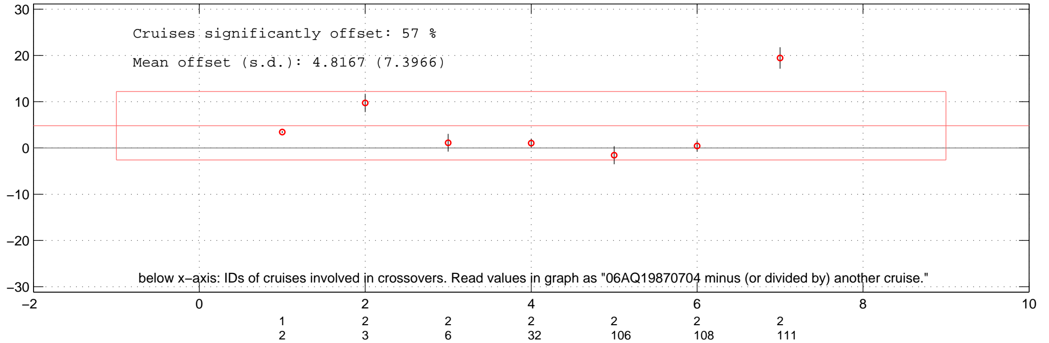
all multiplicative offsets of NO3 of 06AQ19870704 in Favourite-space.
