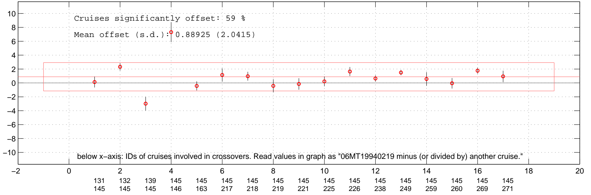
all multiplicative offsets of O2 of 06MT19940219 in Favourite-space.
