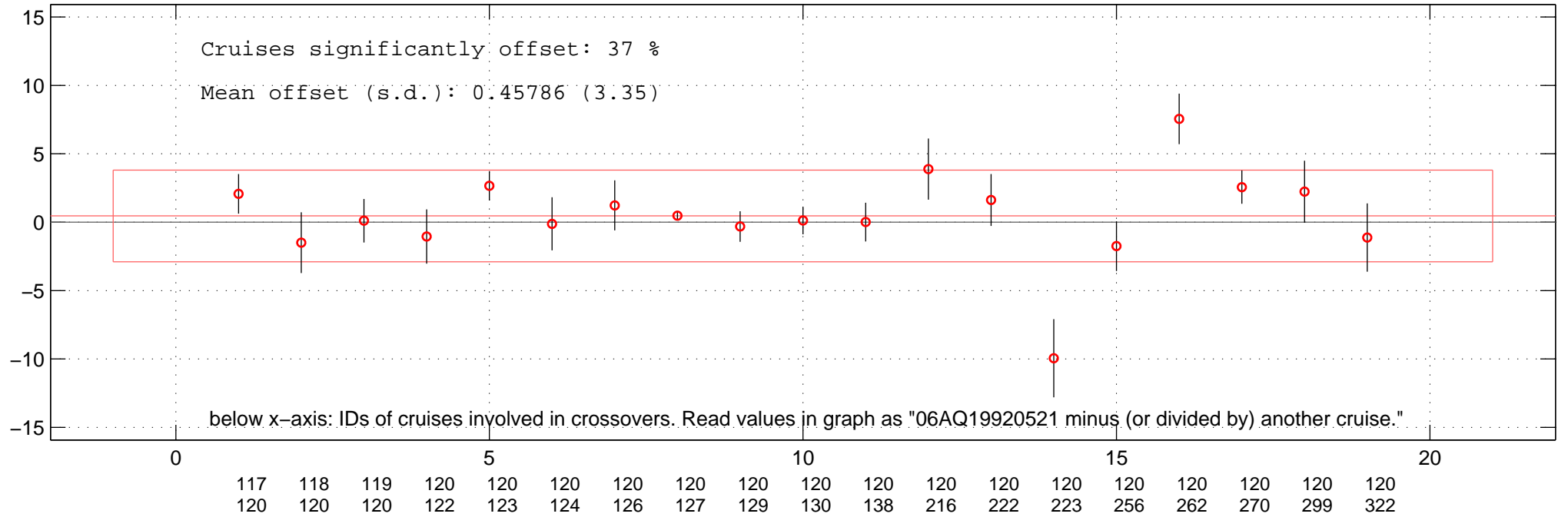
all multiplicative offsets of PO4 of 06AQ19920521 in Favourite-space.
