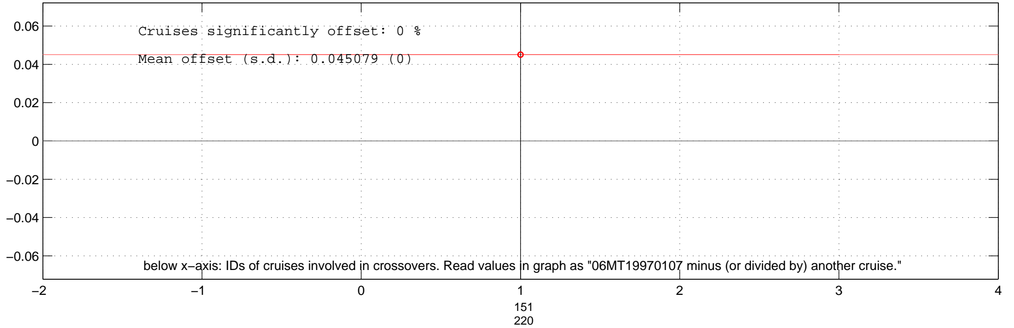
all multiplicative offsets of PO4 of 06MT19970107 in Favourite-space.
