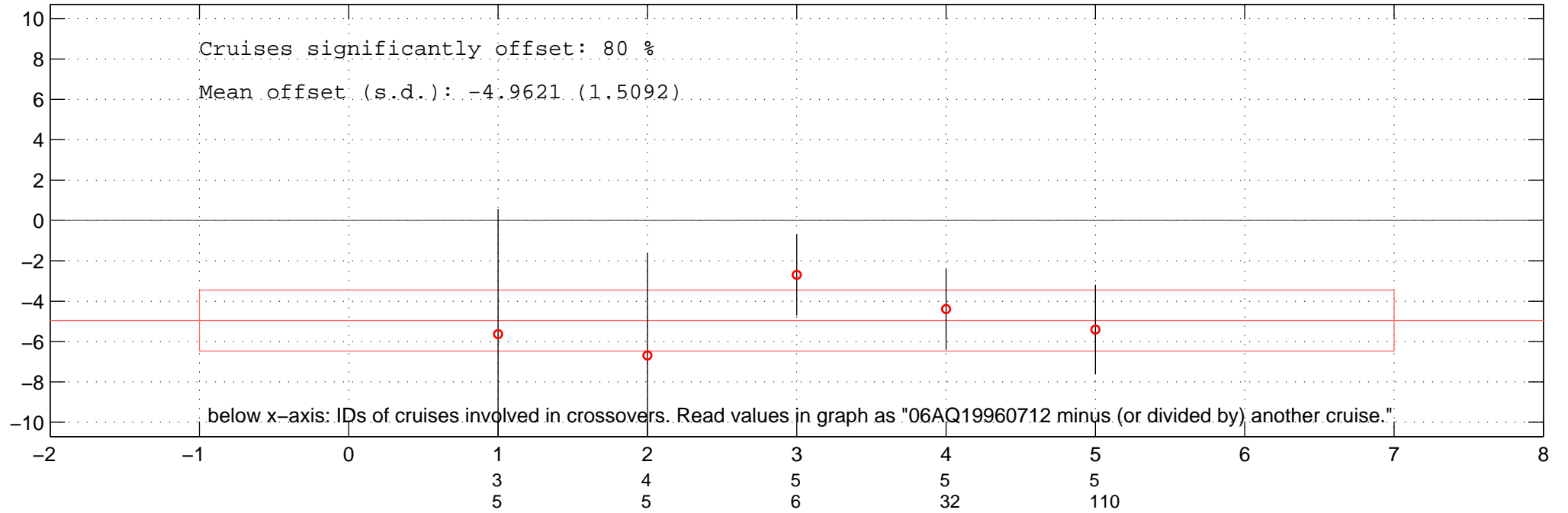
all multiplicative offsets of PO4 of 06AQ19960712 in Favourite-space.
