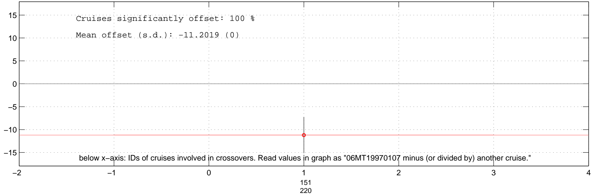
all multiplicative offsets of SIL of 06MT19970107 in Favourite-space.
