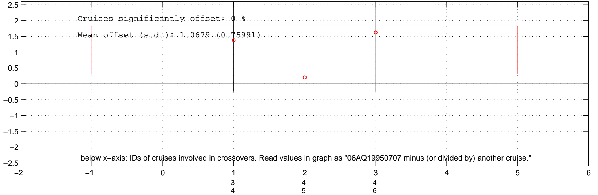
all multiplicative offsets of SIL of 06AQ19950707 in Favourite-space.
